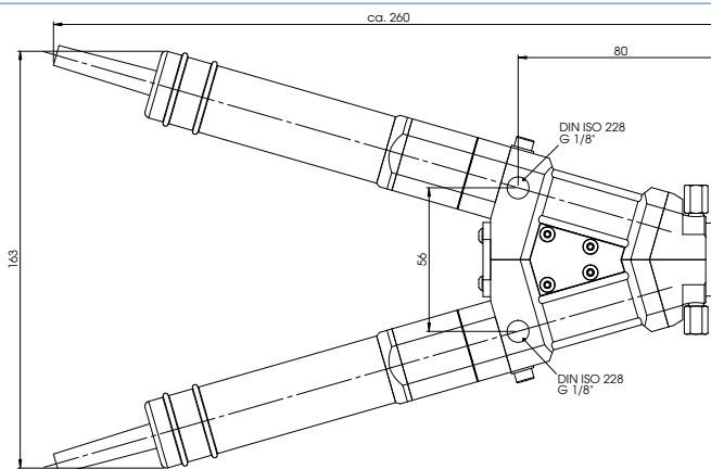
Fig.:Side view
